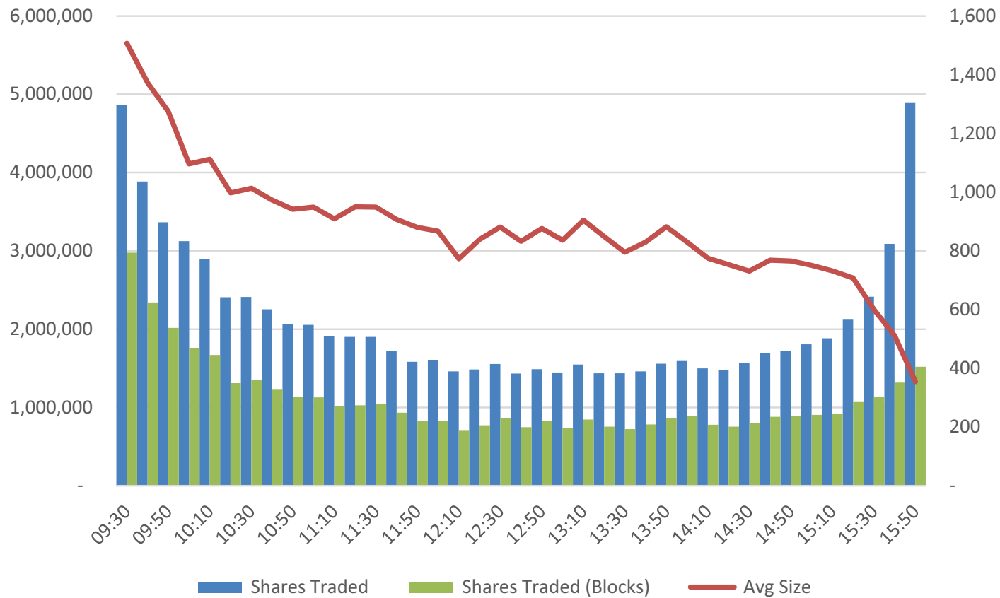
BIDS Trade Volume by Time of Day (10 Minute Time Slices)
